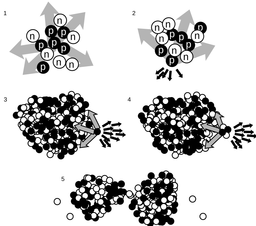
q / 1. The forces cancel. 2. The forces don't cancel. 3. In a heavy nucleus, the large number of electrical repulsions can add up to a force that is comparable to the strong nuclear attraction. 4. Alpha emission. 5. Fission.
